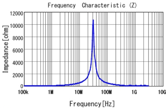
■ 1267AY-100M |Z|
